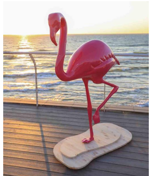
Using its Massivit 1800 3D Printer, SuperSize produced an eye-catching 1.8m / 5.9ft tall flamingo for luxury private event
